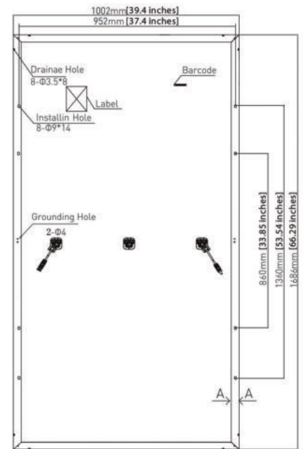
Back View
